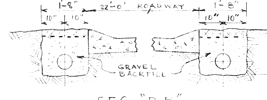
SEC. "B-B" SCALE 1/2" = 1'-0"
