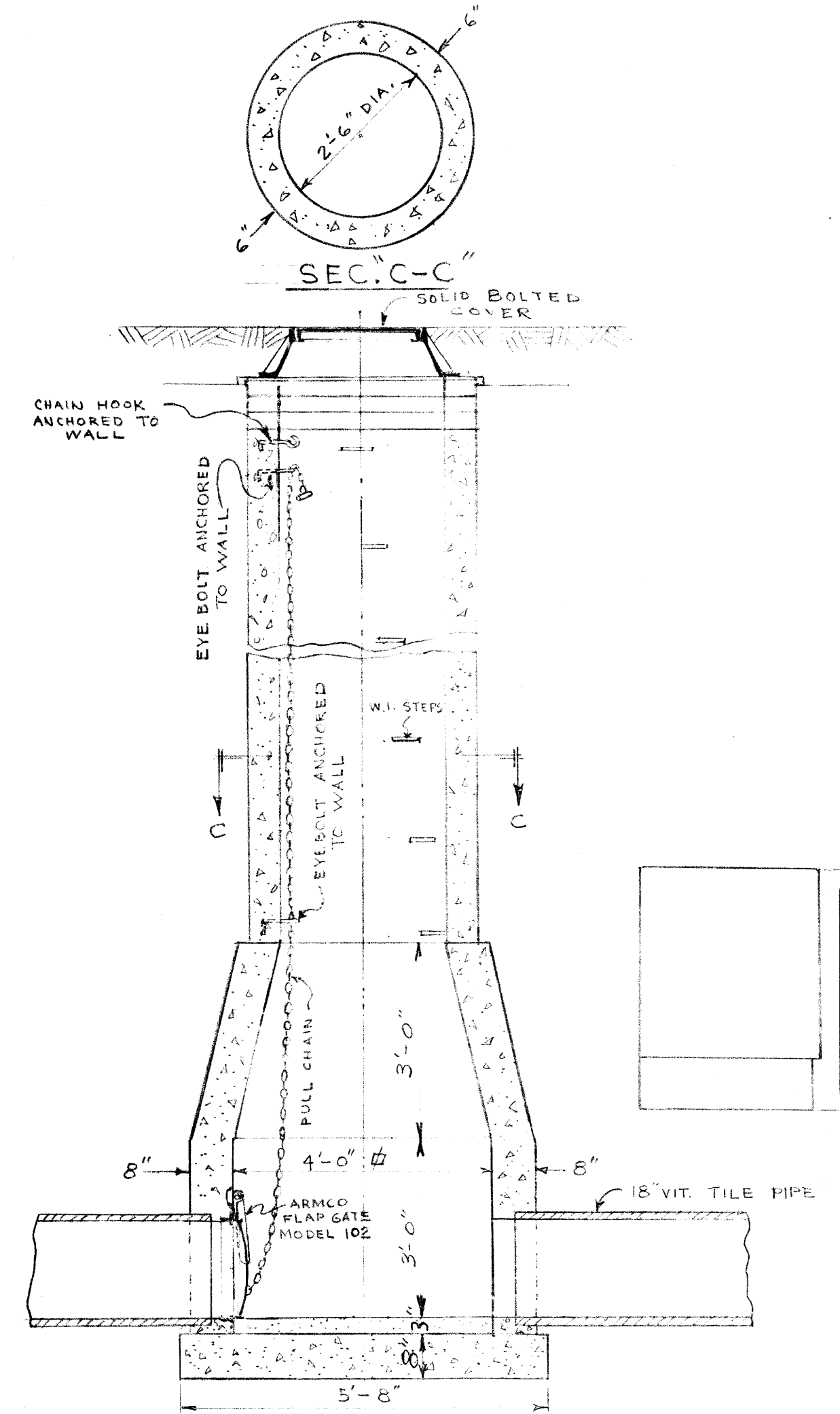
DETAIL OF M.H. WITH FLAP GATE SCALE 1/2" = 1'-0"
