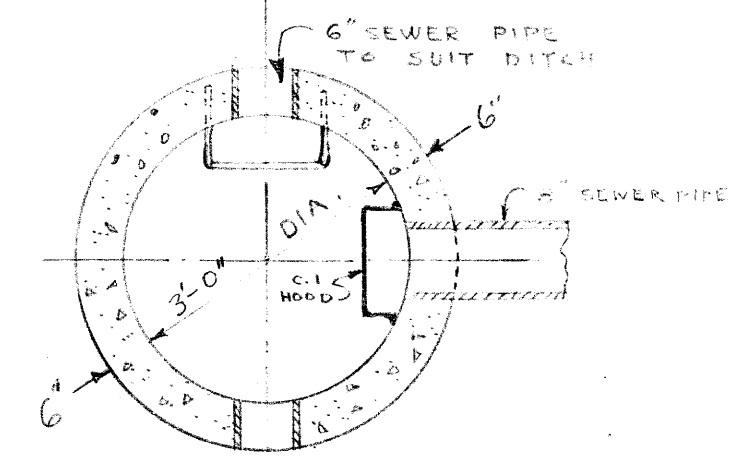
DETAIL OF M.H. WITH FLAP GATE SCALE 1/2" = 1'-0"
